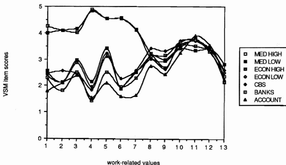
Exhibit 9.1. VSM trends within and between disciplines
