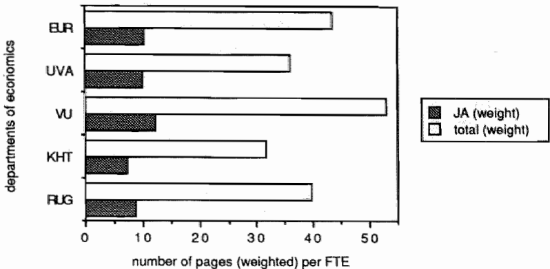
Exhibit 7.1. Departmental Productivity in Dutch Economics
