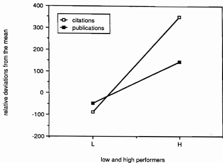
Exhibit 7.4. Subsample Performance Differences
